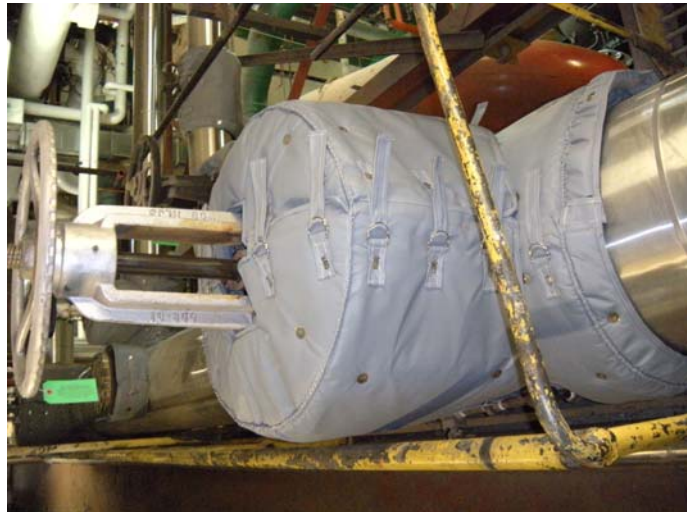
( 400 DN ) 16" 300# HP Steam Gate Valve
