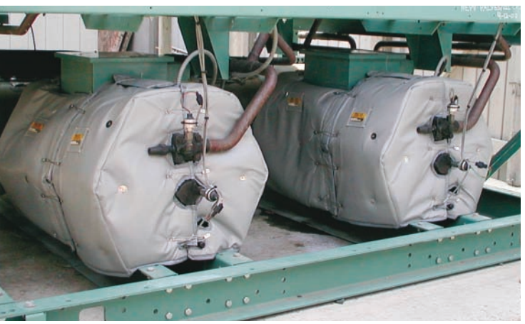
RECIP. COMPRESSOR ENCLOSURE Design: LT250A-VP - 1.0" thick 4 dBA Reduction
